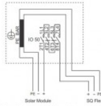
Fig. 1 Wiring diagram, one DC conductor earthed
